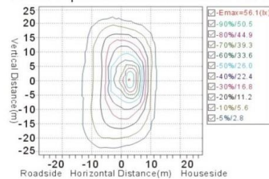
Plane Equivalent Illuminance Curve
