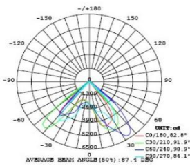
Chart 7: Polar Candela Distribution
