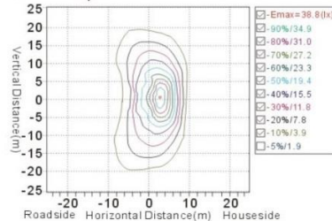
Plane Equivalent Illuminance Curve
