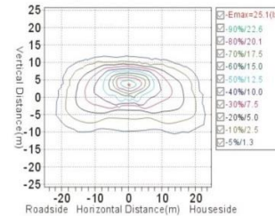
Plane Equivalent Illuminance Curve
