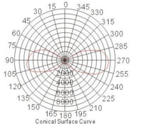
Peak Point Conical Surface Curve
