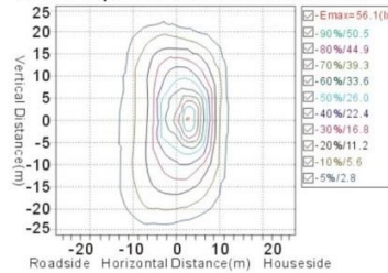
Plane Equivalent Illuminance Curve
